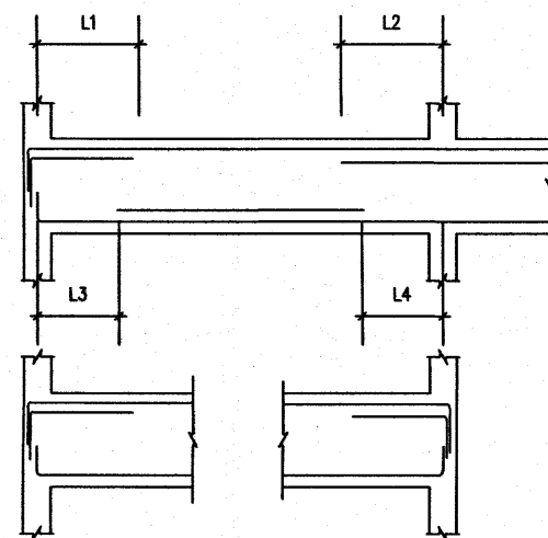
Typical detail 1
