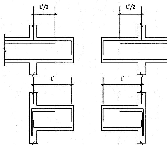
Typical detail 5
