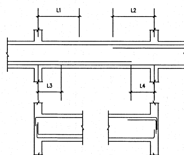
Typical detail 4
