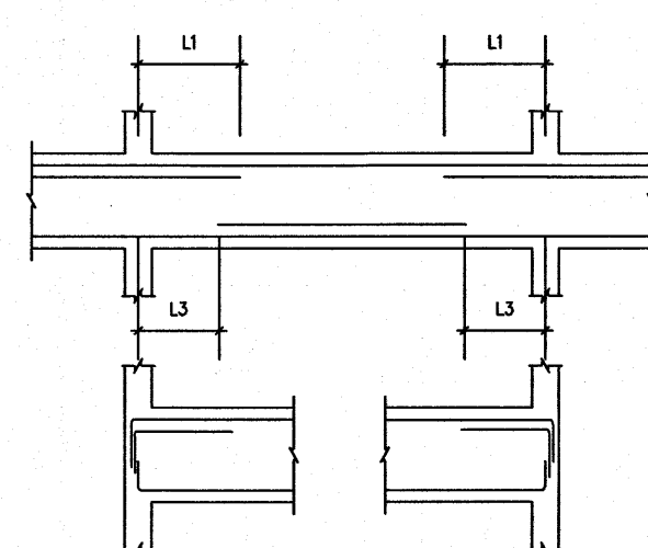
Typical detail 2
