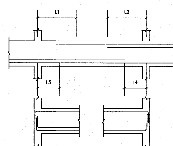
Typical detail 4
