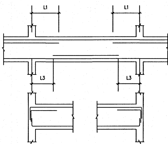
Typical detail 2
