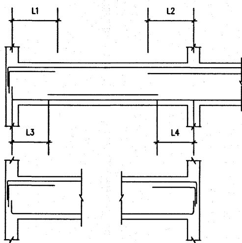
Typical detail 1
