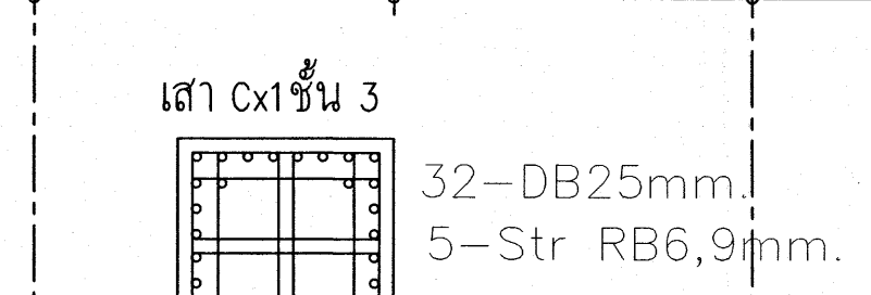
SECTION 0.60x0.60m.
