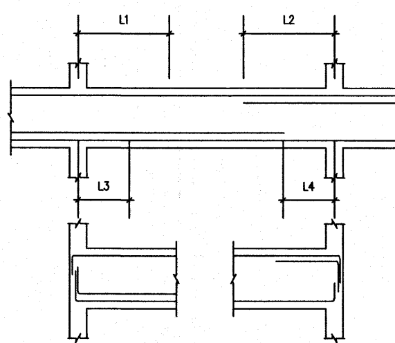
Typical detail 4
