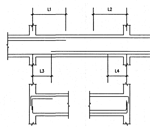
Typical detail 3
