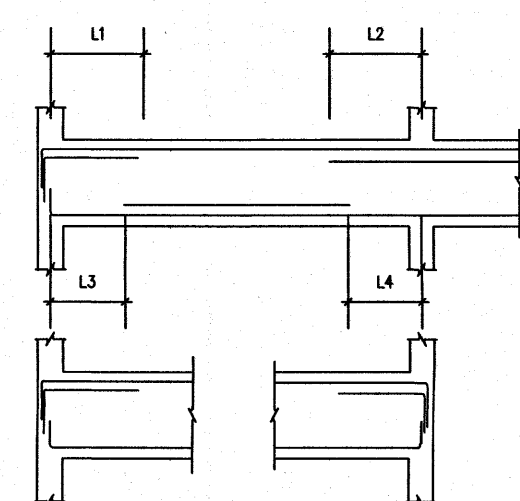
Typical detail 1
