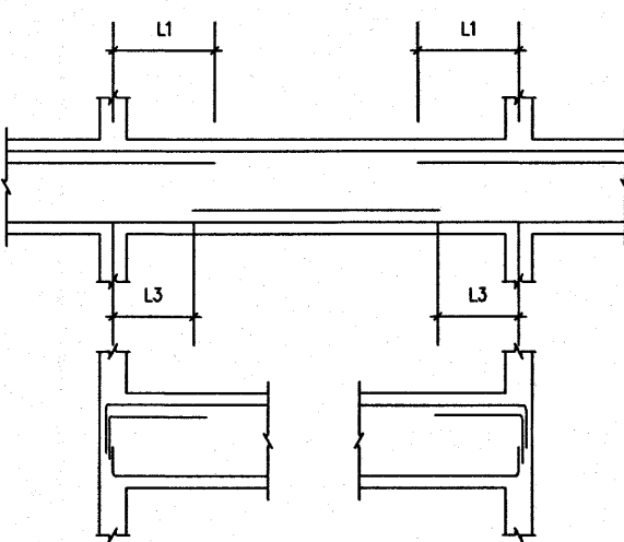
Typical detail 2
