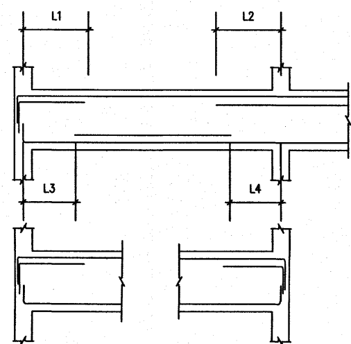
Typical detail 1
