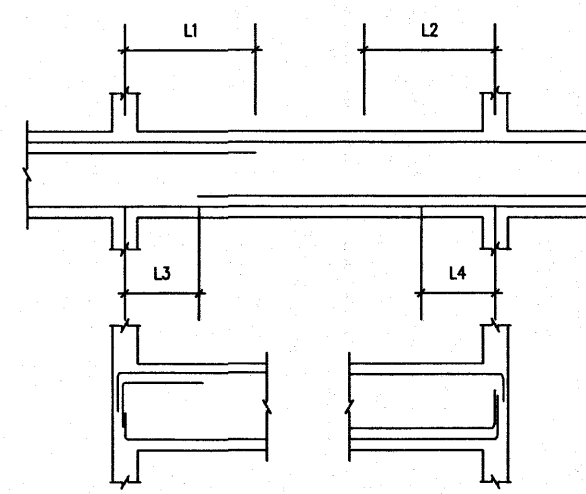
Typical detail 3
