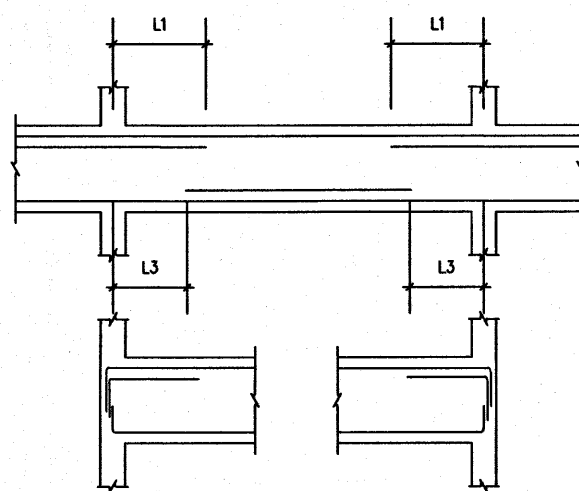
Typical detail 2
