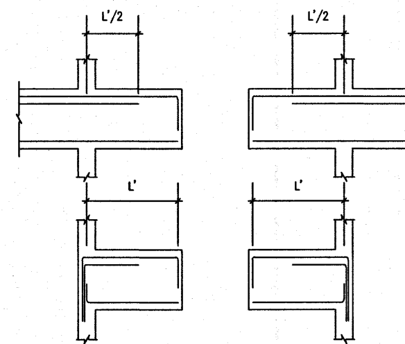
Typical detail 5
