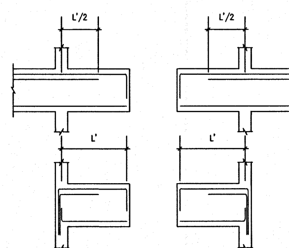
Typical detail 5
