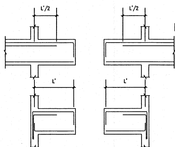
Typical detail 5
