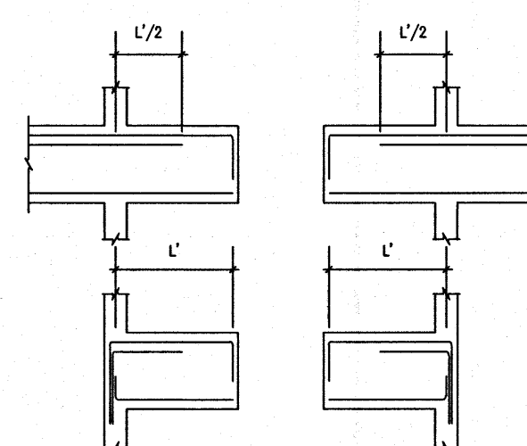
Typical detail 5
