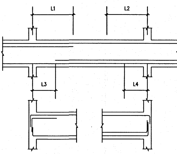
Typical detail 3
