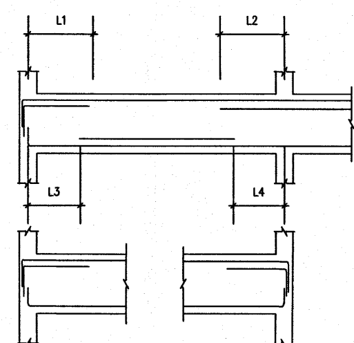
Typical detail 1
