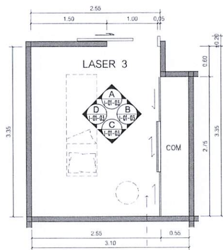
KEY PLAN 1:50 LASER 3
