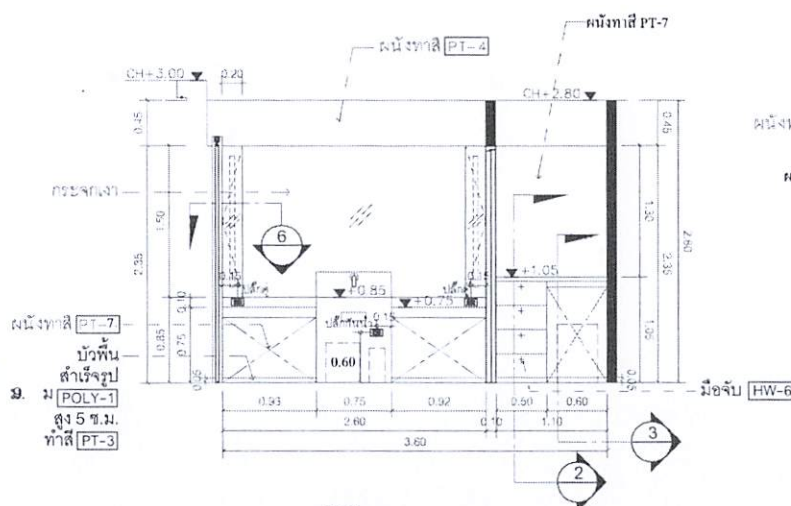
C ELEVATION 1:50 (07-00-00)
