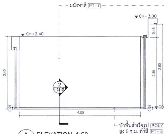
A ELEVATION 1:50 I-01-05 LASER 5
