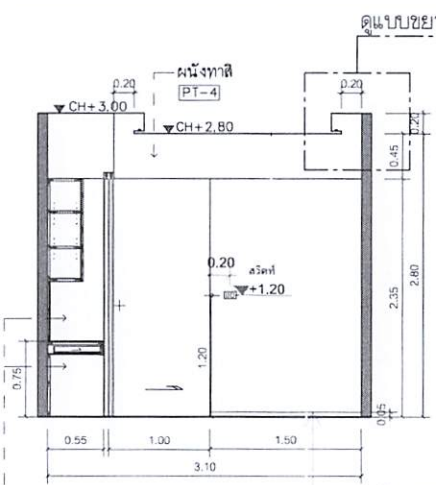
C ELEVATION 1:50 LASER 1
