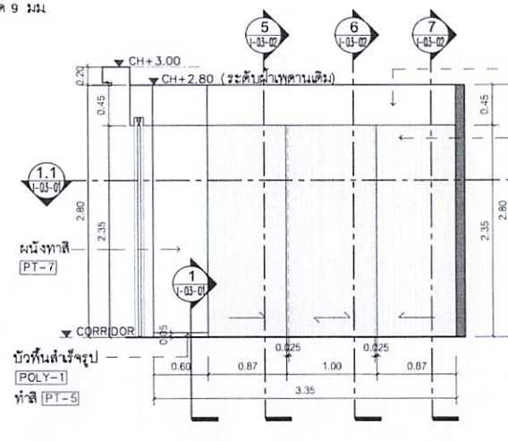
B ELEVATION 1:50 LASER 3
