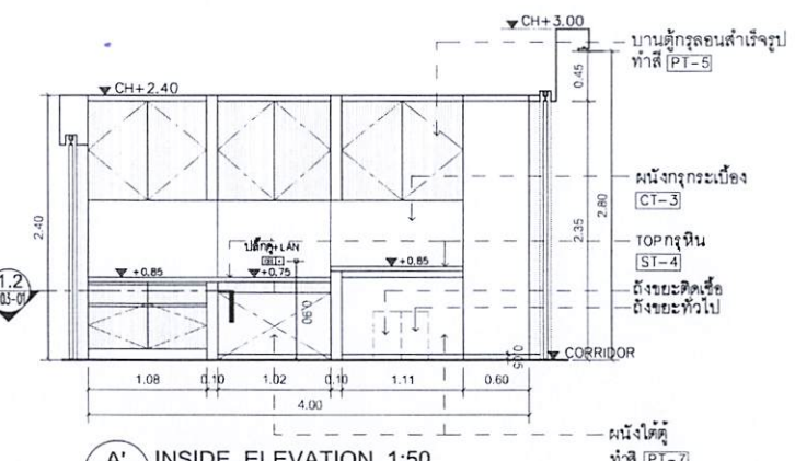
A' INSIDE ELEVATION 1:50 I-01-06 LASER 6
