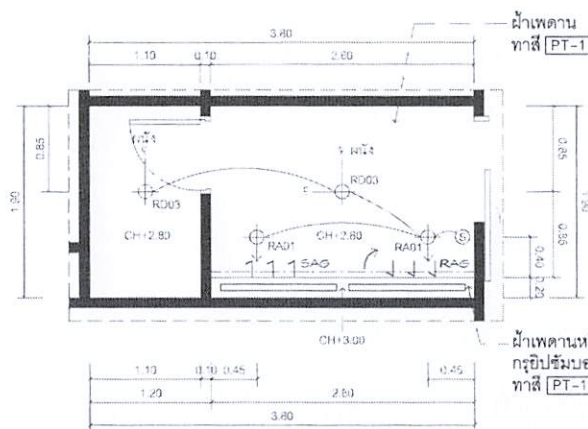
REFLECTED CEILING PLAN 1:50
