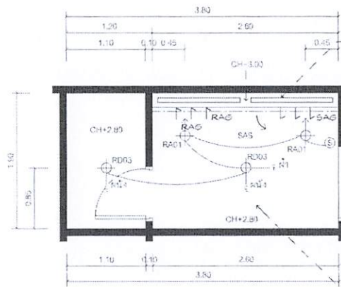
REFLECTED CEILING PLAN 1:50 MEN
