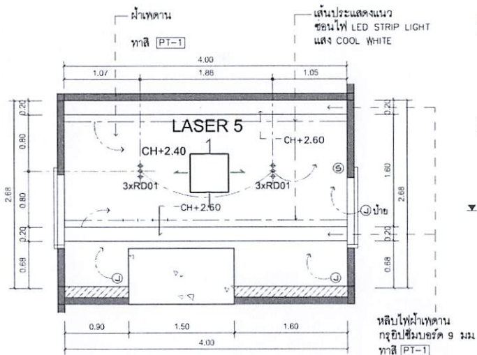
REFLECTED CEILING PLAN 1:50 LASER 5
