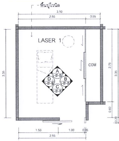
KEY PLAN 1:50 LASER 1
