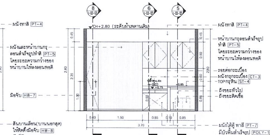
C' INSIDE ELEVATION 1:50 I-01-04 LASER 4
