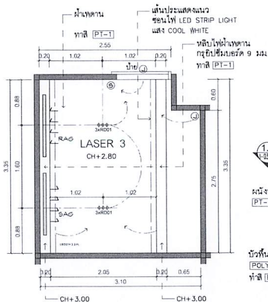
REFLECTED CEILING PLAN 1:50 LASER 3
