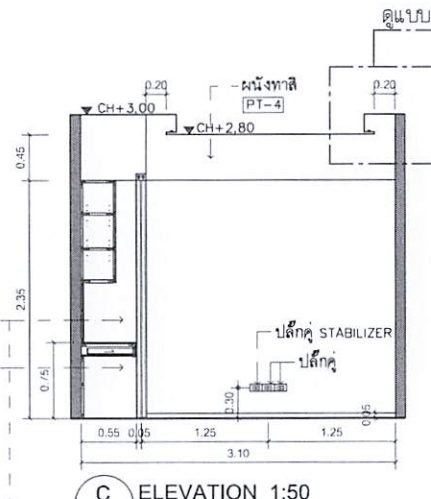
C ELEVATION 1:50 LASER 3
