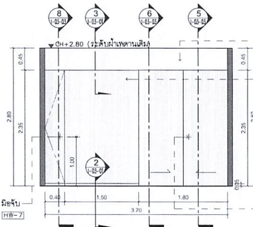
C ELEVATION 1:50 I-01-04 LASER 4
