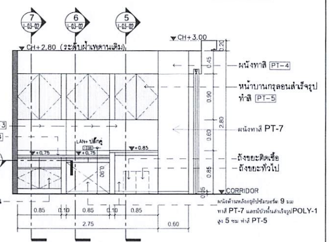
B' INSIDE ELEVATION 1:50 LASER 1
