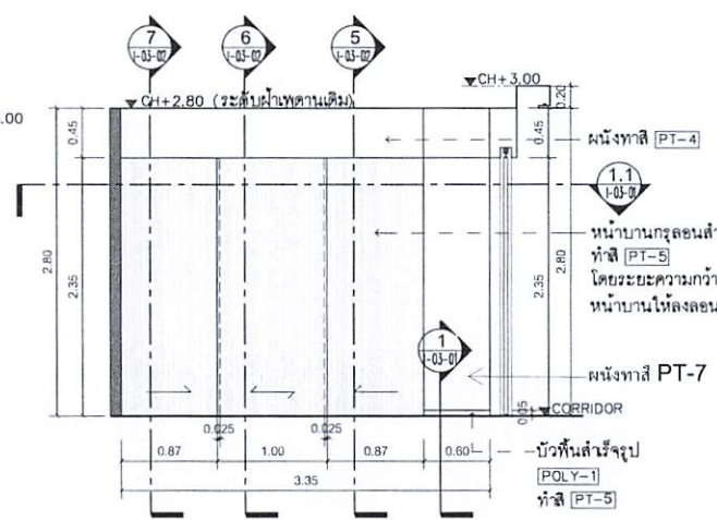
B ELEVATION 1:50 LASER 1
