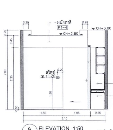
A ELEVATION 1:50 LASER 3
