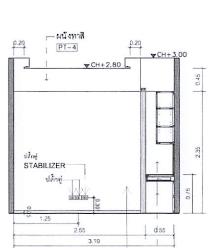
A ELEVATION 1:50 LASER 1
