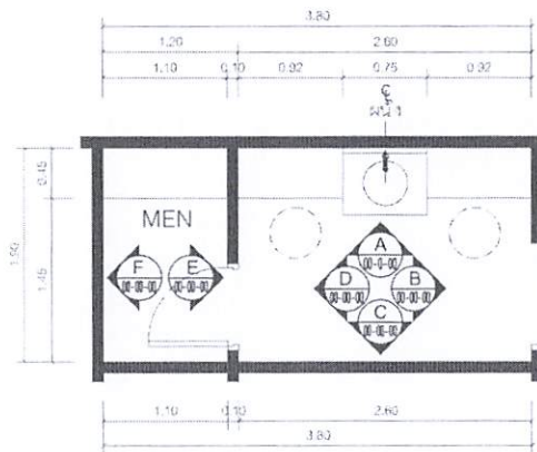
KEY PLAN 1:50 MEN
