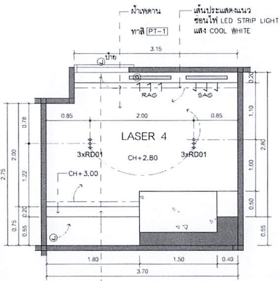
REFLECTED CEILING PLAN 1:50 LASER 4
