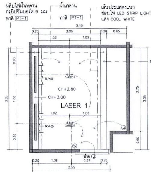
REFLECTED CEILING PLAN 1:50 LASER 1
