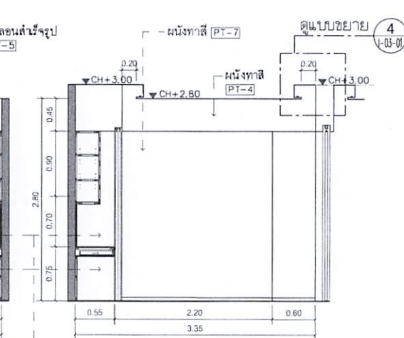
D ELEVATION 1:50 I-01-04 LASER 4
