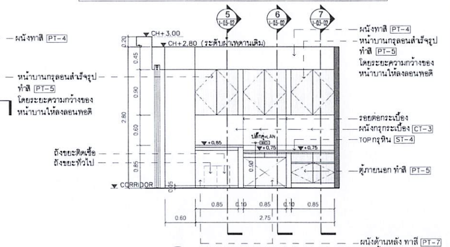
B' INSIDE ELEVATION 1:50 LASER 3
