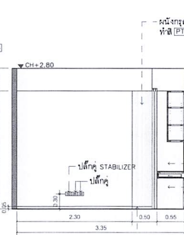
B ELEVATION 1:50 I-01-04 LASER 4
