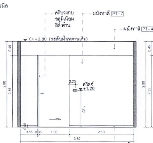
A ELEVATION 1:50 I-01-04 LASER 4
