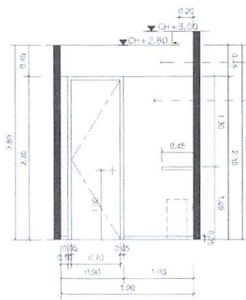
E ELEVATION 1:50 G-01-04
