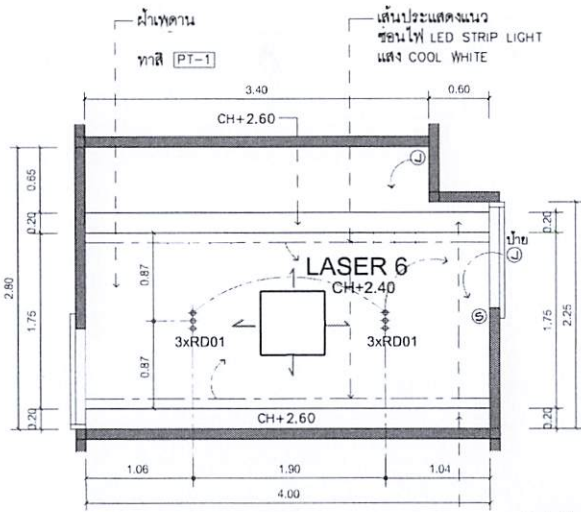
REFLECTED CEILING PLAN 1:50 LASER 6
