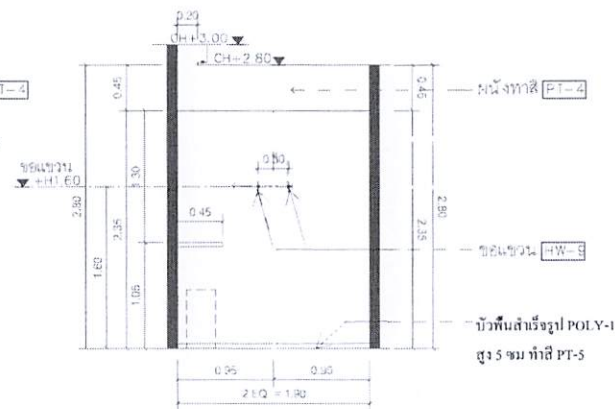
F ELEVATION 1:50 G-01-04
