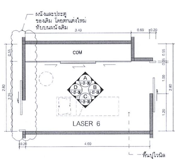
KEY PLAN 1:50 LASER 6
