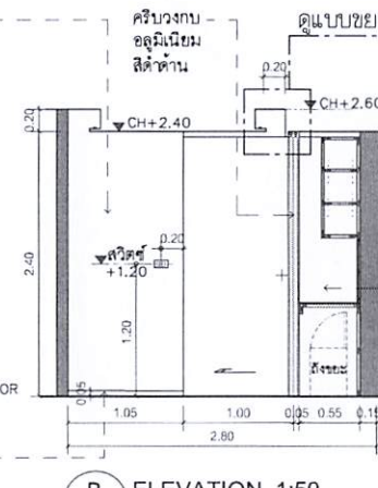
B ELEVATION 1:50 I-01-05 LASER 5
