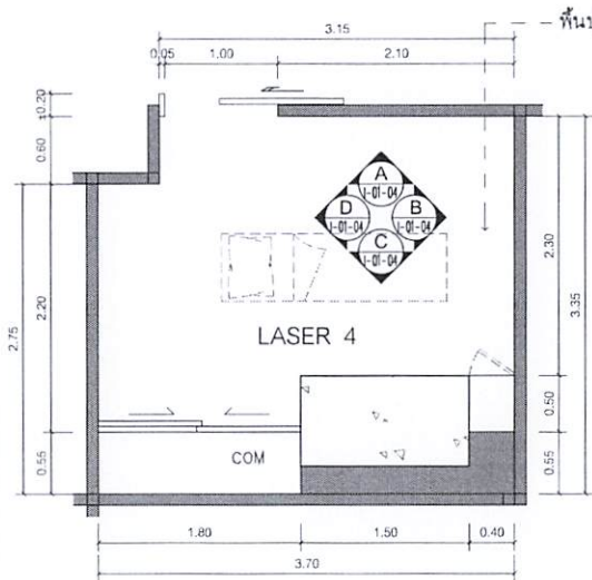
KEY PLAN 1:50 LASER 4
