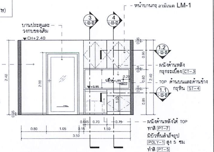
D INSIDE ELEVATION 1:50 OPERATION 1
