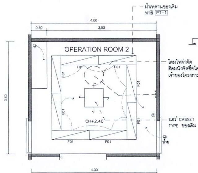
REFLECTED CEILING PLAN 1:50 OPERATION 2
