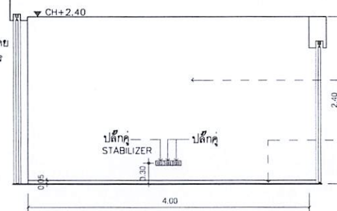
C ELEVATION 1:50 I-01-02 OPERATION 2
