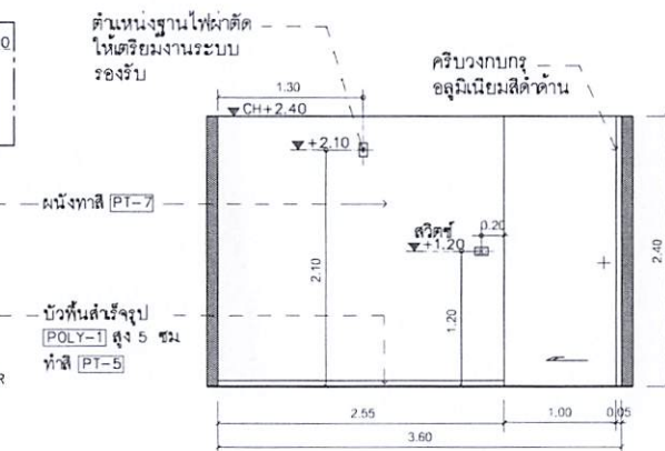
B ELEVATION 1:50 I-01-02 OPERATION 2
