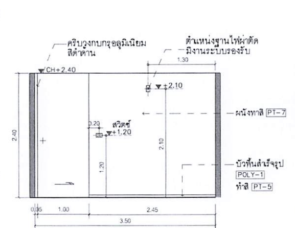
B ELEVATION 1:50 OPERATION 1
