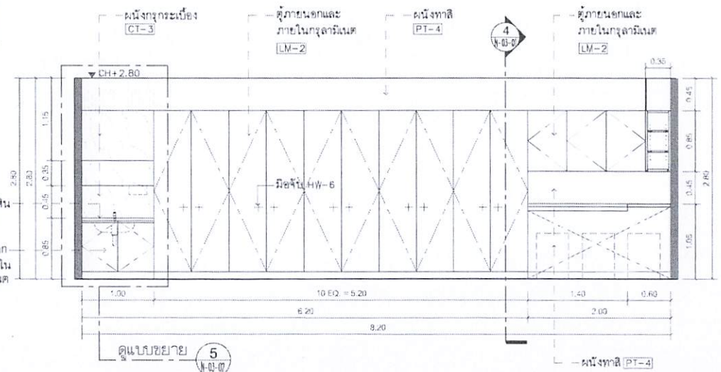
C ELEVATION 1:50 STORAGE 1
