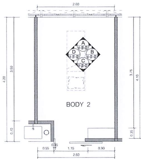
KEY PLAN 1:50 BODY 2
