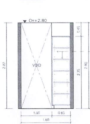
B ELEVATION 1:50 STORAGE 1
