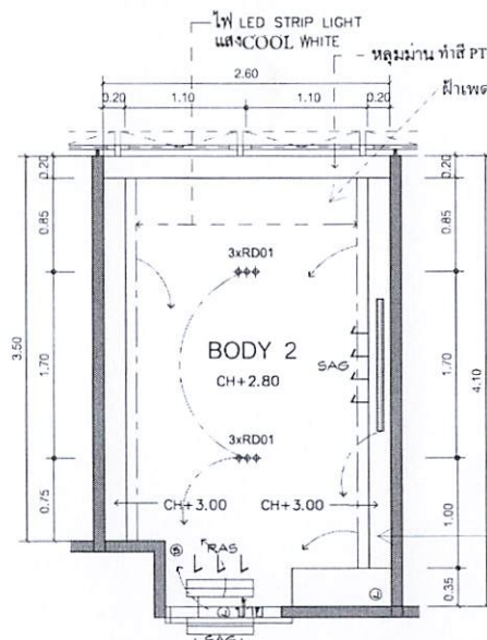
REFLECTED CEILING PLAN 1:50 BODY 2
