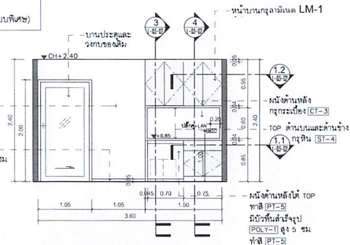
D ELEVATION 1:50 I-01-02 OPERATION 2
