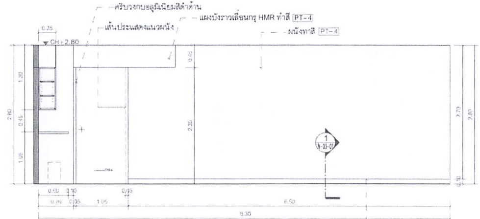
A ELEVATION 1:50 STORAGE 1
