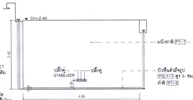
C INSIDE ELEVATION 1:50 OPERATION 1
