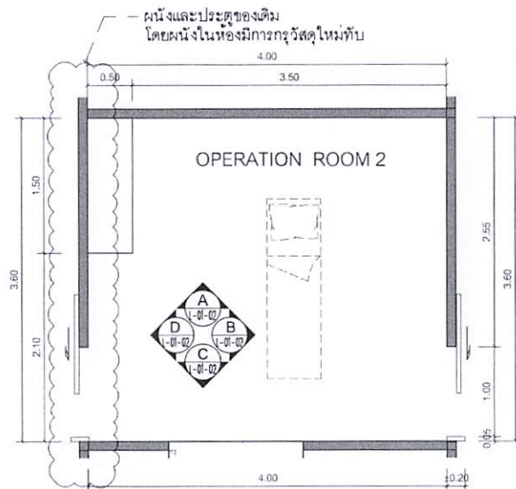
KEY PLAN 1:50 OPERATION 2
