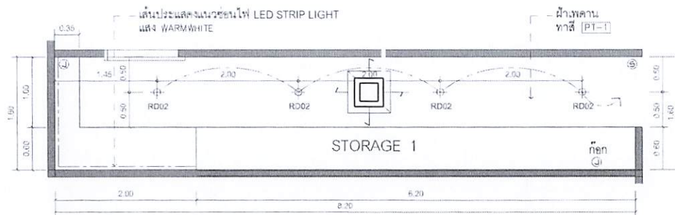
REFLECTED CEILING PLAN 1:50 STORAGE 1
