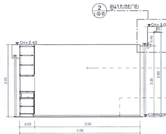
A ELEVATION 1:50 I-01-02 OPERATION 2
