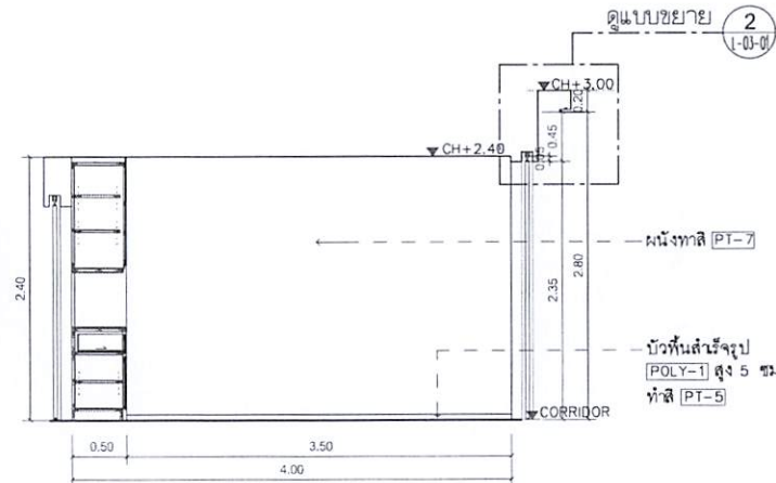
A ELEVATION 1:50 OPERATION 1
