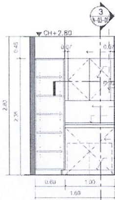
D ELEVATION 1:50 STORAGE 1
