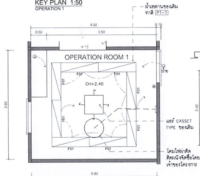
REFLECTED CEILING PLAN 1:50 OPERATION 1
